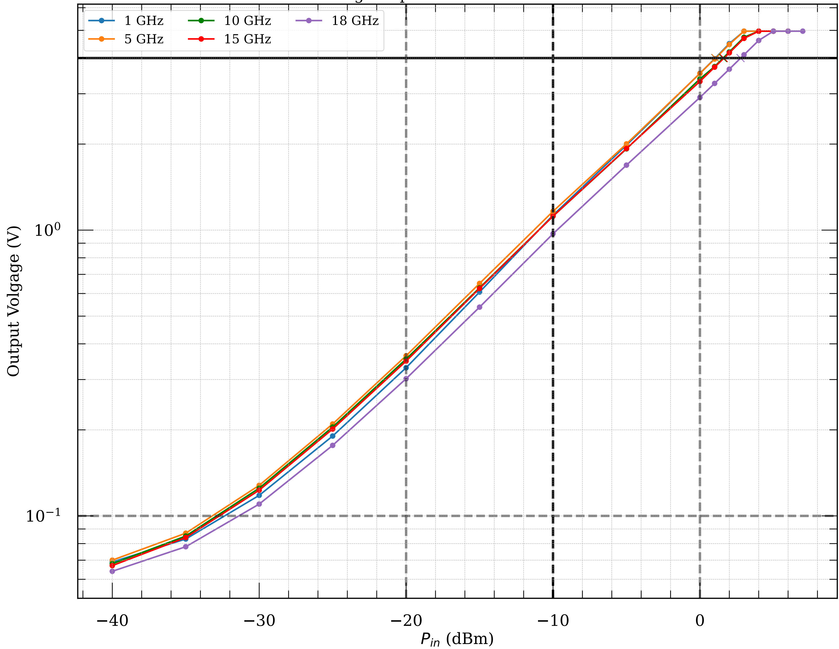
Measured voltage-to-power curve of detector module039
